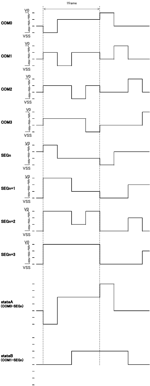
Figure 14. LCD waveform at frame inversion (1/3bias)
