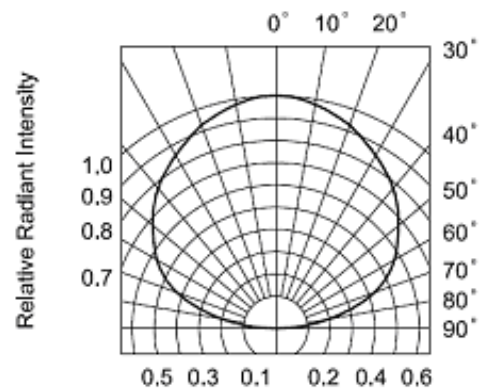
FIG.6 RADIATION DIAGRAM
