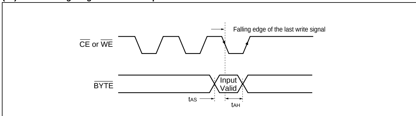
(14) \overline{\text{BYTE}} Timing Diagram for Write Operations
