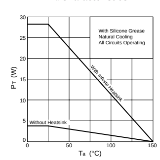
Pr-Ta Characteristics
