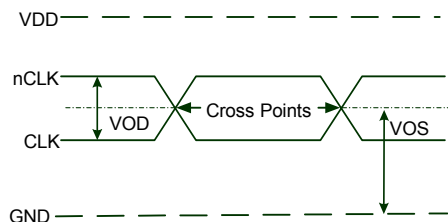
DIFFERENTIAL INPUT LEVEL
