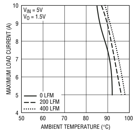
Figure 10. BGA Heatsink
