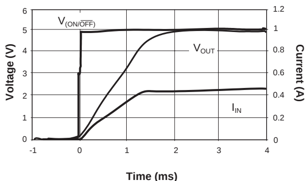
Turn-On Waveforms ( C_{IN} = 1\mu F ; C_{OUT} = 0.1\mu F ; V_{IN} = 5V )
