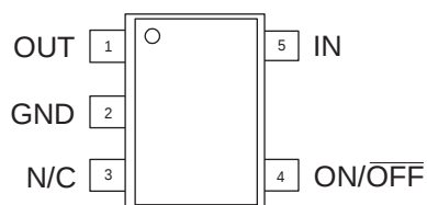
SOT23-5 (SOT25) (Top View)
