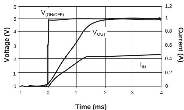
Turn-On Waveforms ( C_{IN} = 1\mu F ; C_{OUT} = 10\mu F ; V_{IN} = 5V )
