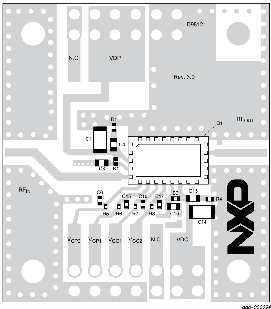
Figure 2. AFSC5G40E38 Reference Circuit Component Layout
