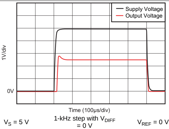
Figure 21. Start-Up Response
