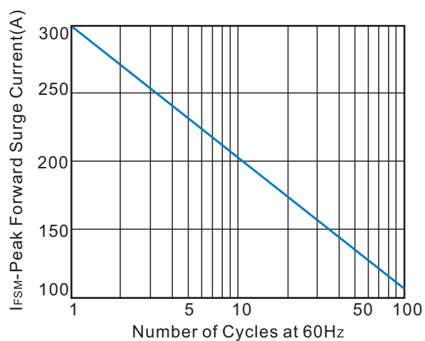
Fig.6 Maximum Non-repetitive Forward Surge
