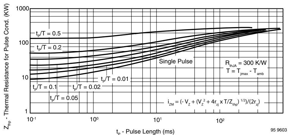
Figure 10. Thermal Response
