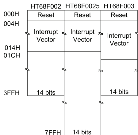
Program Memory Structure
