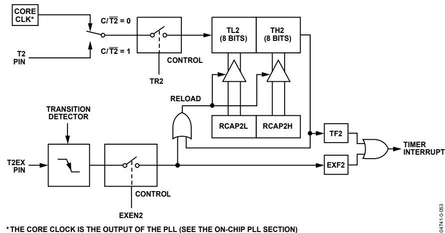
Figure 56. Timer/Counter 2, 16-Bit Autoreload Mode
