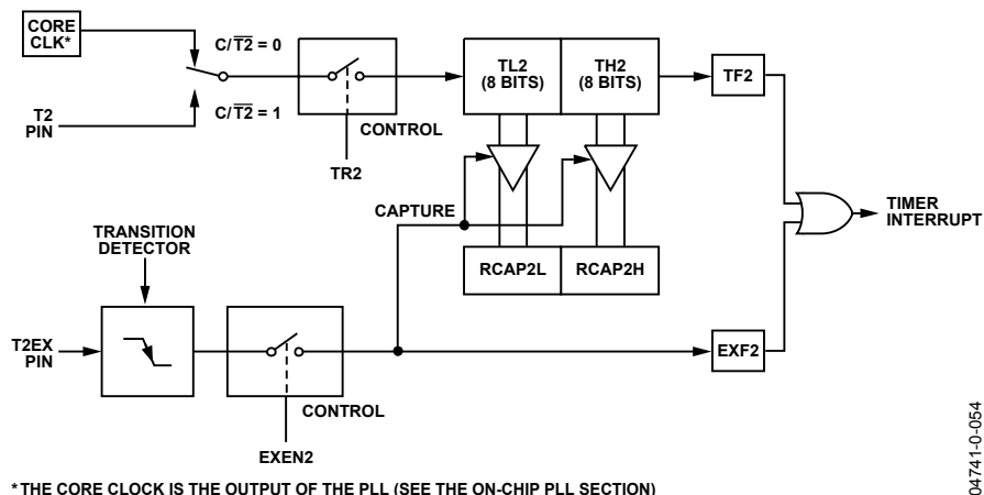
Figure 57. Timer/Counter 2, 16-Bit Capture Mode
