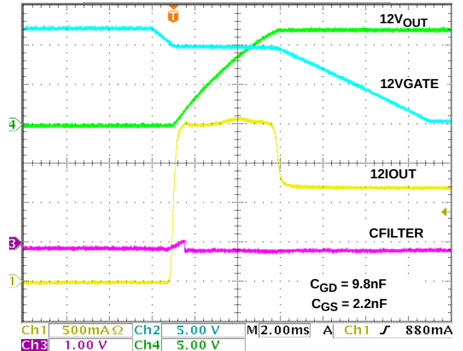
FIGURE 7. ISL6113 12VMAIN START-UP R_{LOAD} = 10\Omega , C_{LOAD} = 470\mu F
