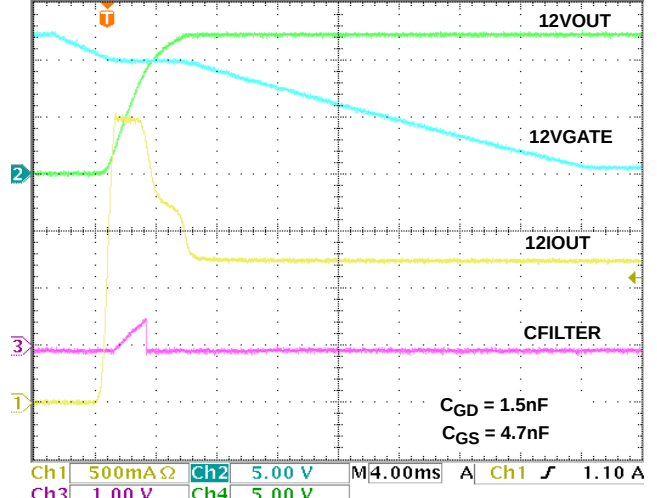
FIGURE 8. ISL6114 12VMAIN START-UP R_{LOAD} = 10\Omega , C_{LOAD} = 470\mu F
