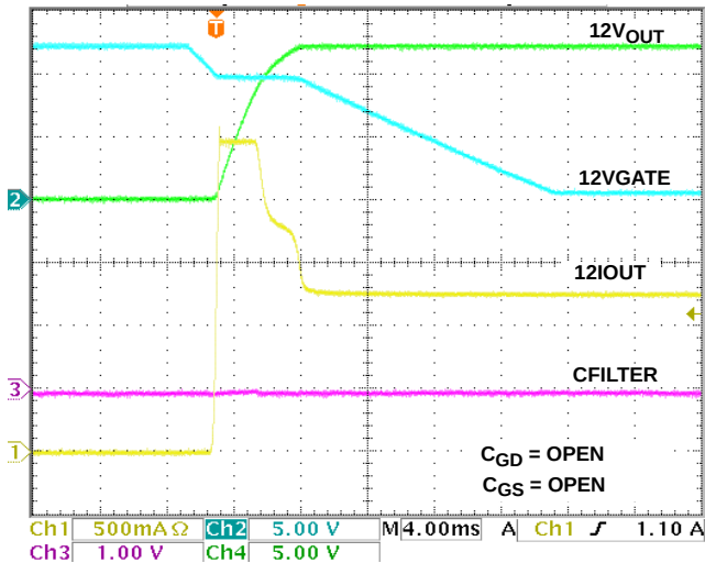
FIGURE 10. ISL6114 12VMAIN START-UP R_{LOAD} = 10\Omega , C_{LOAD} = 470\mu F
