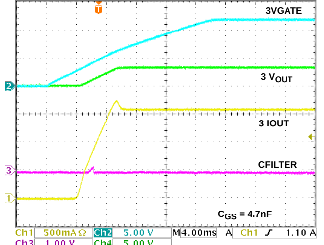
FIGURE 9. ISL6114 3VMAIN START-UP R_{LOAD} = 2\Omega , C_{LOAD} = 470\mu F
