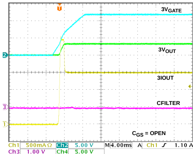
FIGURE 11. ISL6114 3VMAIN START-UP R_{LOAD} = 2\Omega , C_{LOAD} = 470\mu F
