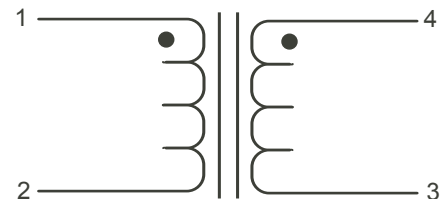
Schematic
