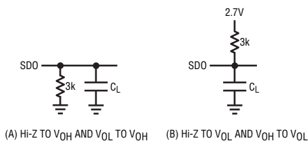
Load Circuits for Access Timing
