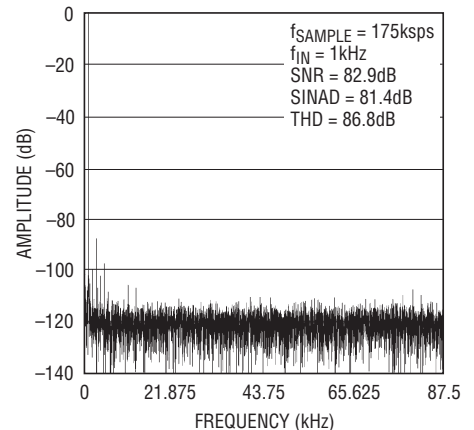
4096 Points FFT Plot ( V_{DD} = 2.7\text{V} , Internal REF)
