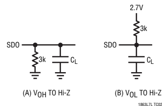
Load Circuits for Output Float Delay
