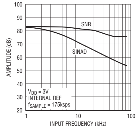
Signal-to-(Noise + Distortion) Ratio vs Input Frequency
