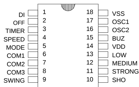
SM3502-B 18PIN
