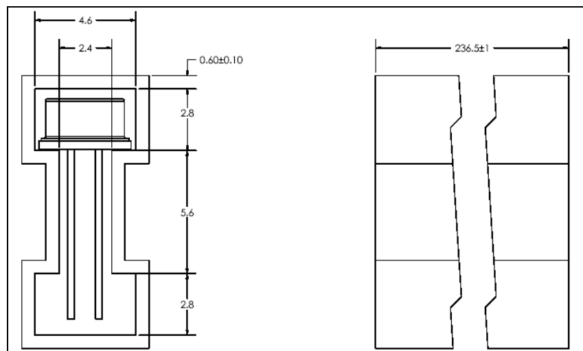
Main dimensions of packing tube
