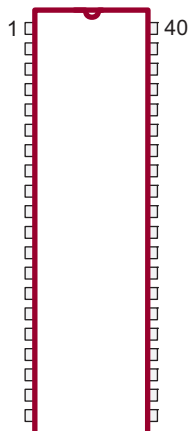
40-lead PDIP (Top view)
