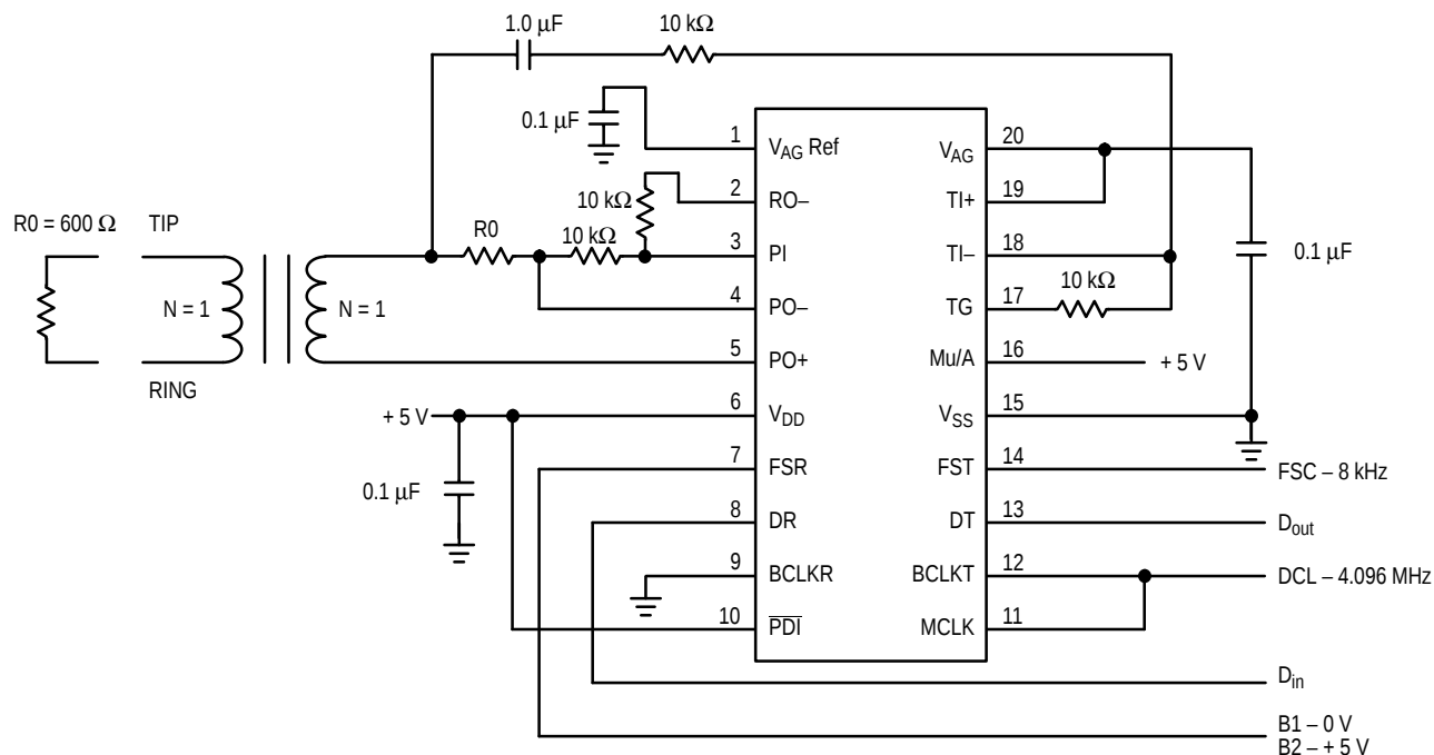
Figure 11. MC145484 Transformer Interface to 600 Ω Telephone Line with GCI Clocking
