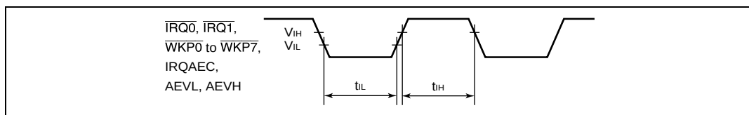
Figure 17.3 Input Timing
