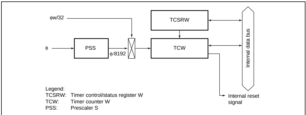
Figure 9.12(1) Block Diagram of Watchdog Timer (H8/38004, H8/38002S Group)
