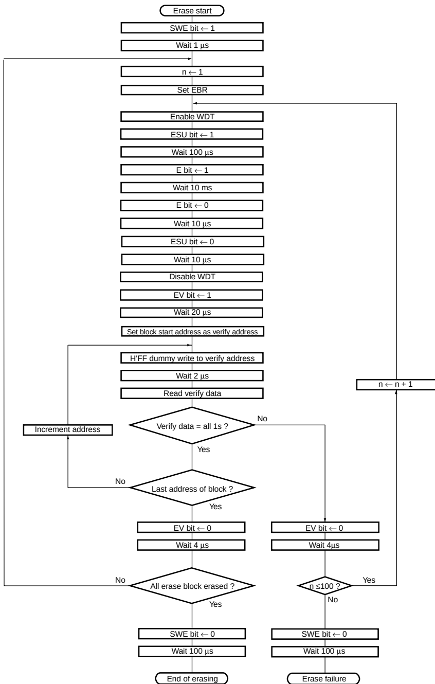
Figure 6.11 Erase/Erase-Verify Flowchart
