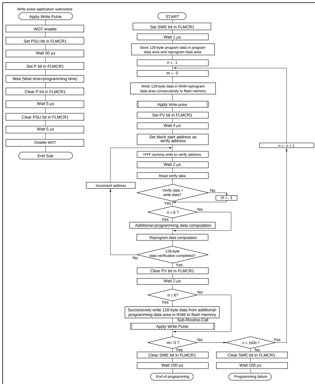
Figure 6.10 Program/Program-Verify Flowchart
