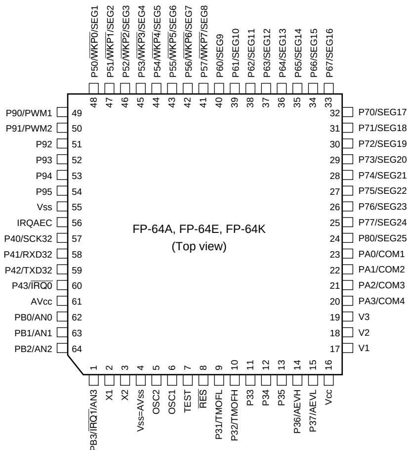
Figure 1.4 Pin Arrangement of H8/3802, H8/38004 and H8/38002S Group (FP-64A, FP-64E, FP-64K)
