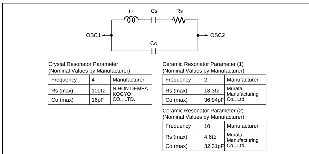
Figure 17.8 Resonator Equivalent Circuit
