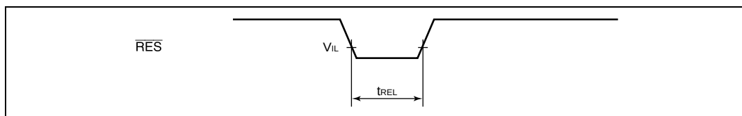
Figure 17.2 RES Low Width Timing
