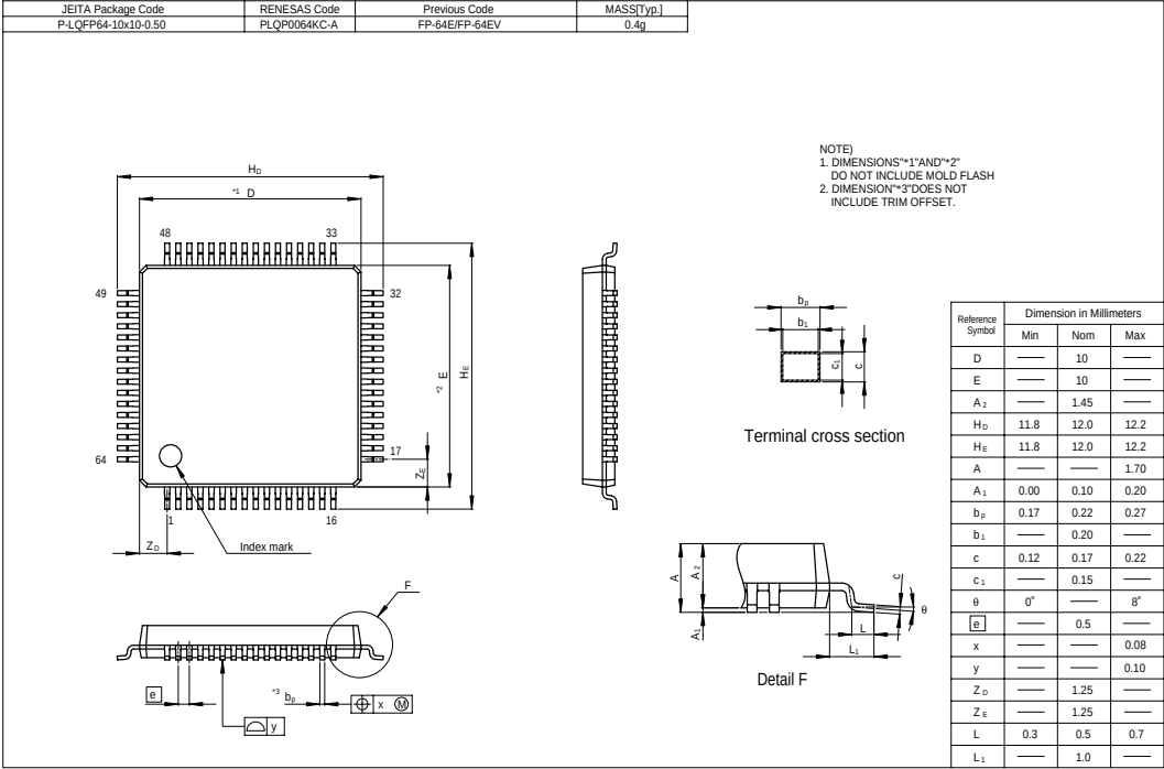
Figure E.2 Package Dimensions (FP-64E)
