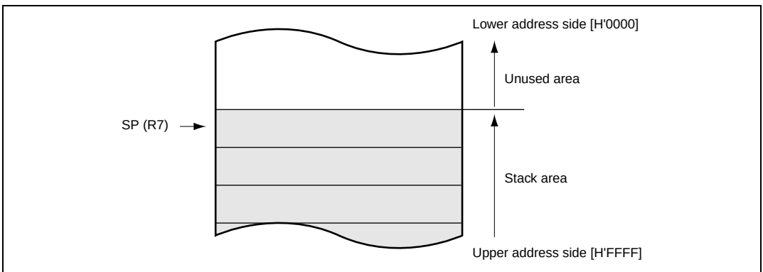
Figure 2.3 Stack Pointer
