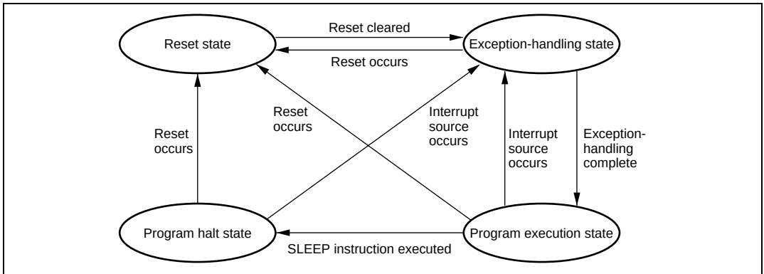
Figure 2.16 State Transitions
