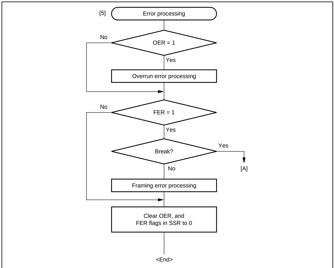
Figure 10.17 Sample Multiprocessor Serial Reception Flowchart (2)
