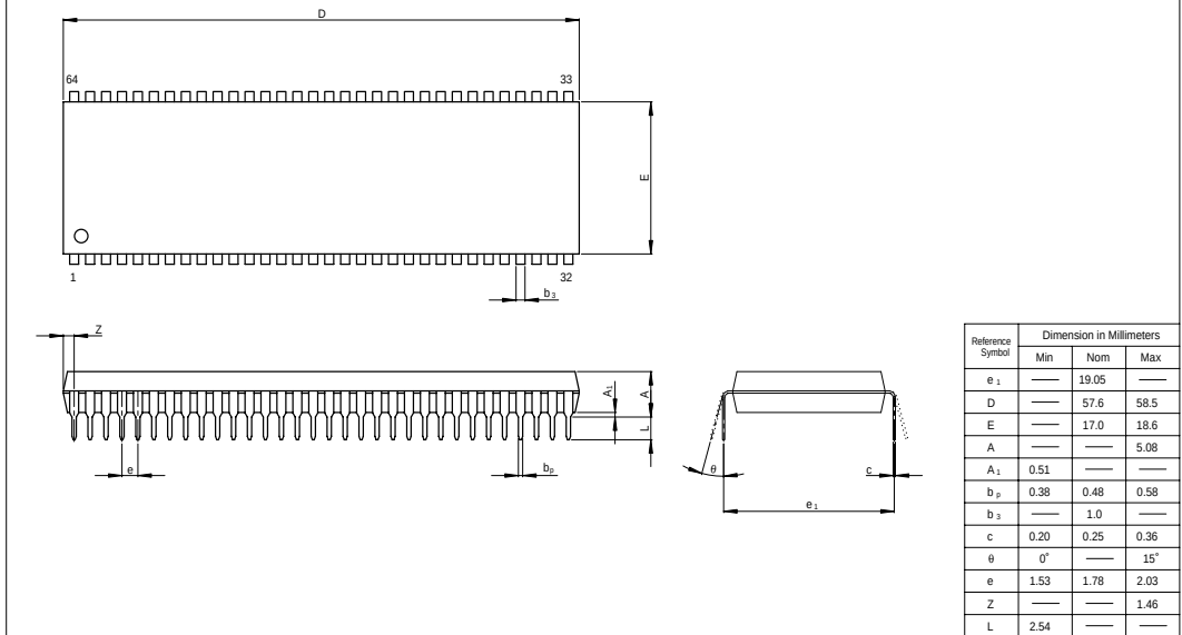
Figure E.4 Package Dimensions (DP-64S)
