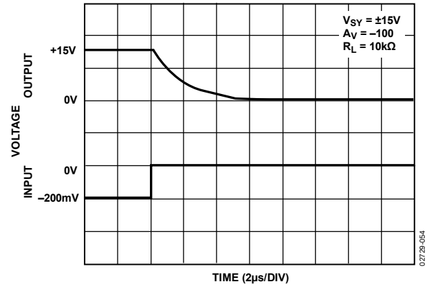
Figure 43. Negative Overload Recovery
