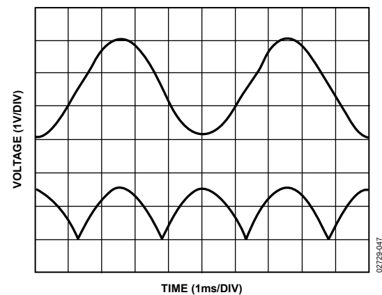
Figure 51. Full-Wave Rectifier Signal (OUT B in Figure 49)
