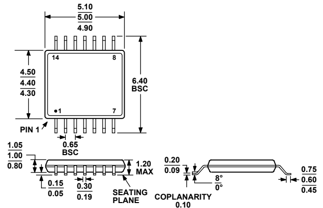
Figure 60. 14-Lead Thin Shrink Small Outline Package [TSSOP] (RU-14)
