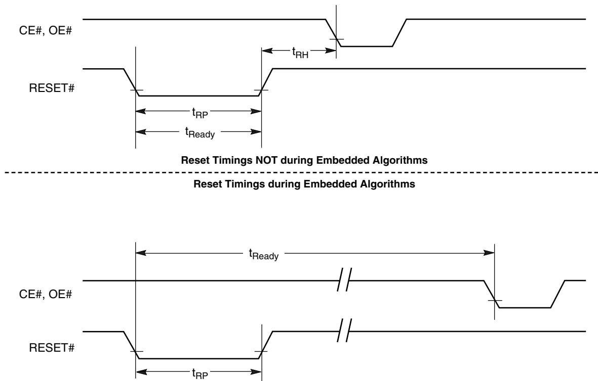
Figure 17. Reset Timings
