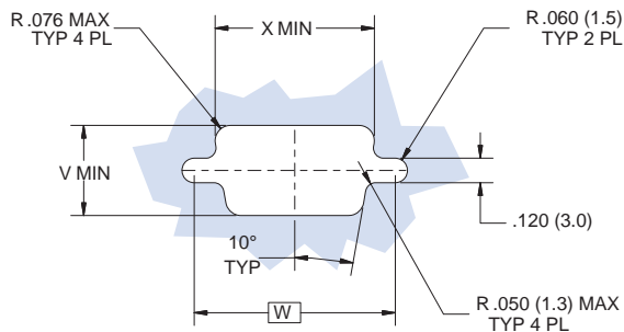
REAR PANEL MOUNT CUTOUT RECOMMENDATIONS AS VIEWED FROM FRONT FACE OF PANEL
