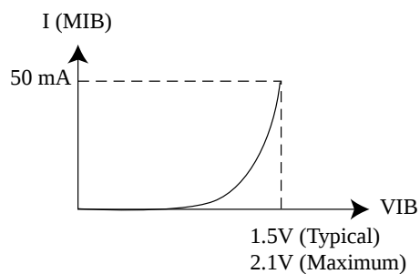
Figure 4: Control Signals VIP and VIB
