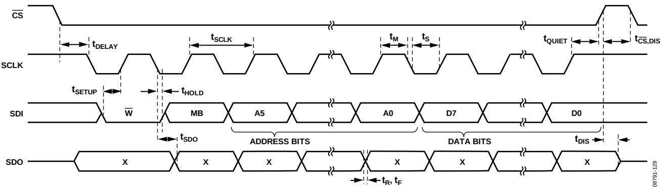
Figure 24. SPI 4-Wire Write
