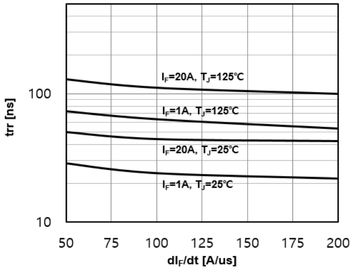
Fig. 3) Typical Reverse recovery time
