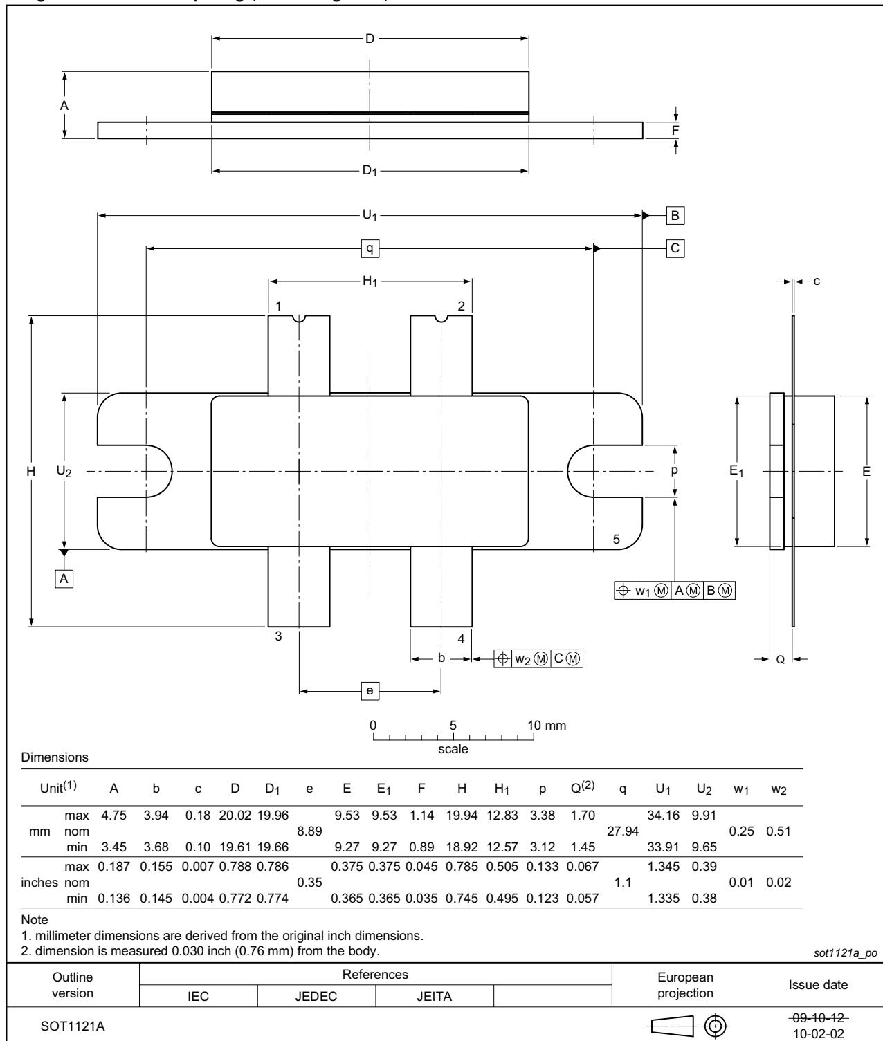
Fig 8. Package outline SOT1121A
