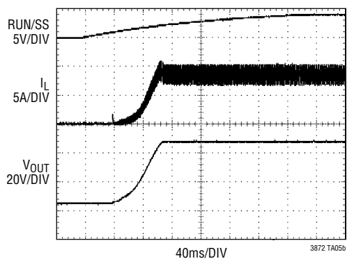
Soft-Start
