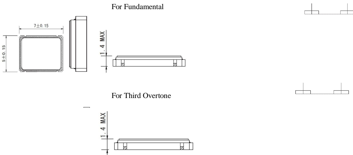
Suggested solder pad layout
