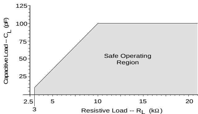
Figure 3. Maximum Loading
