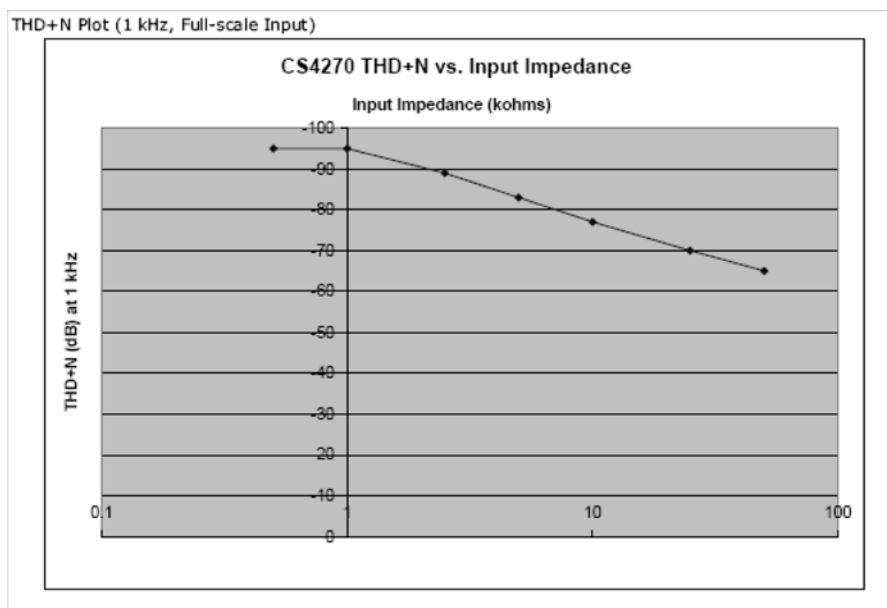
Figure 16. A/D THD+N Performance vrs. Input Source Resistance
