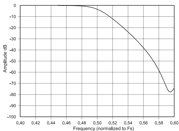
Figure 29. DAC Double-Speed Transition Band
