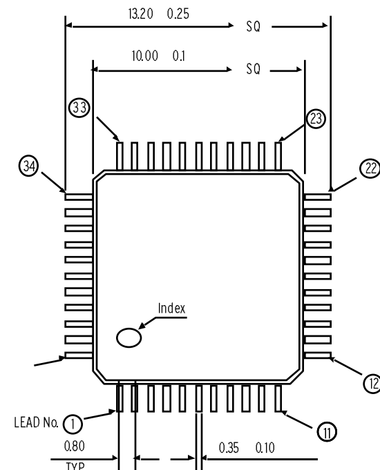
Fig. 5 QFP44 package
