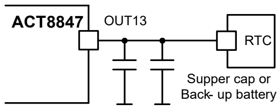
Typical Application of RTC LDO
