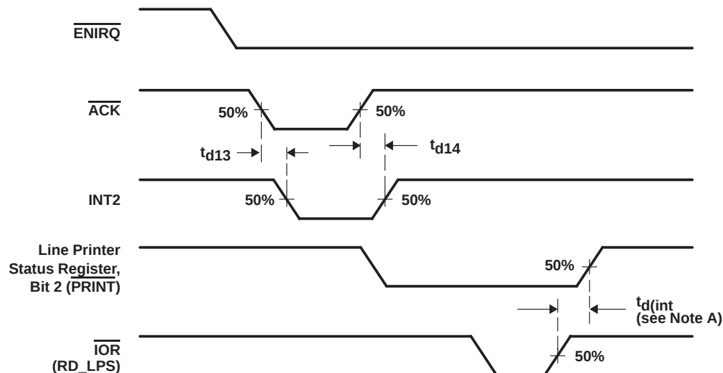
Figure 16. Parallel Port AT Mode Timing ( \overline{\text{ENIRQ}} = Low) Waveforms
