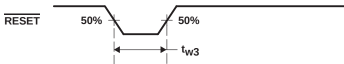
Figure 18. \overline{\text{RESET}} Voltage Waveform
