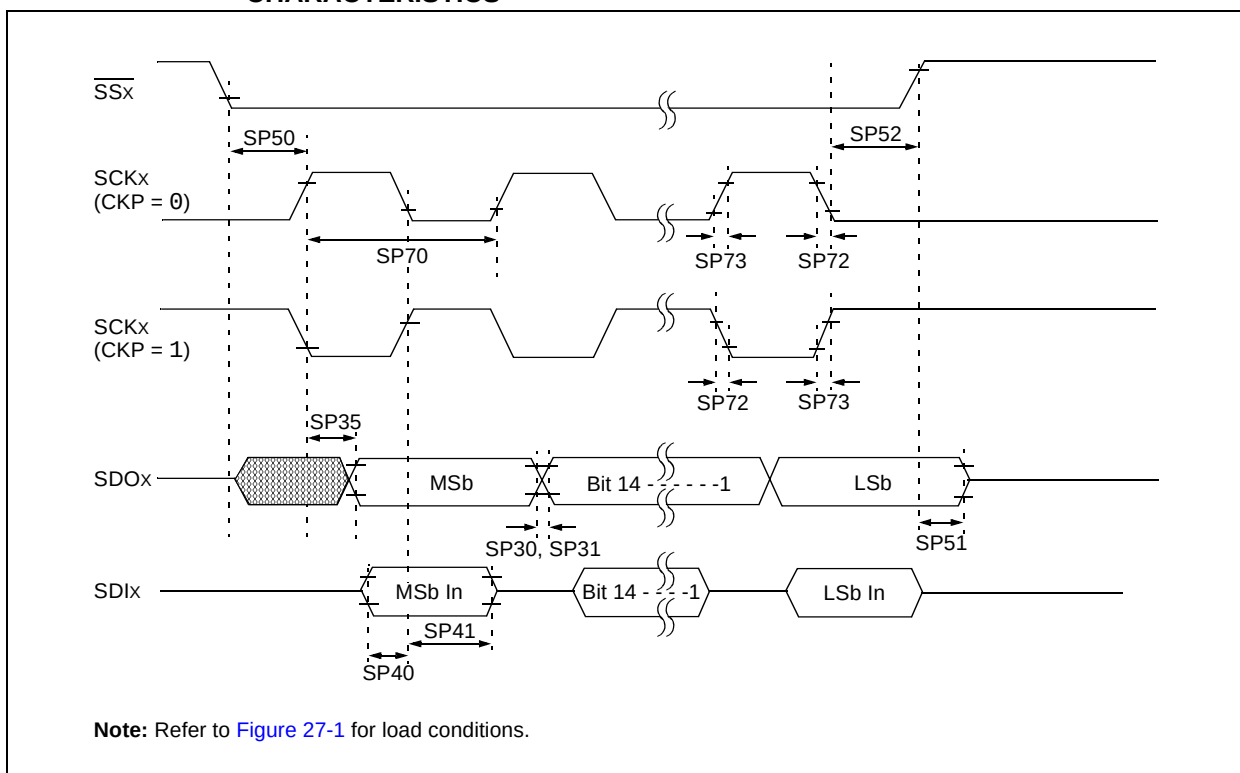
FIGURE 27-18: SPIx SLAVE MODE (FULL-DUPLEX, CKE = 0, CKP = 0, SMP = 0) TIMING CHARACTERISTICS
