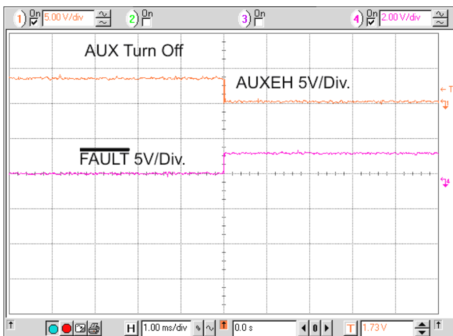
Figure 24. AUX Disable Turn Off - \overline{\text{FAULT}}
