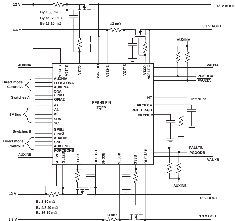
Application Diagram
