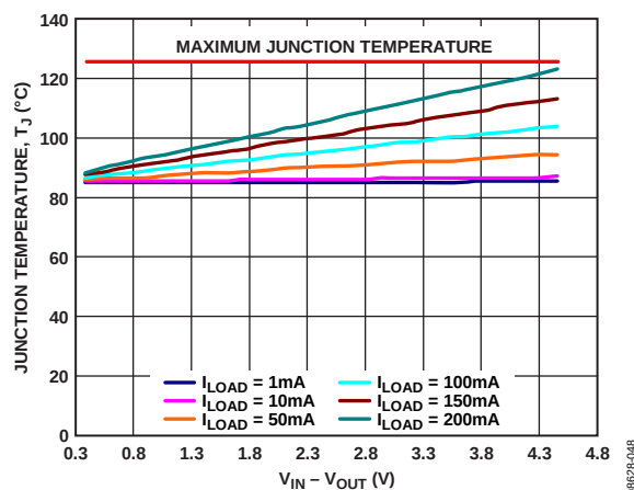
Figure 50. TSOT, T_A = 85^{\circ}\text{C}
