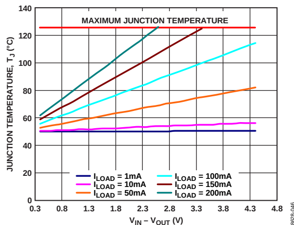
Figure 48. 100 mm 2 of PCB Copper, T_{SOT} , T_A = 50^{\circ}\text{C}
