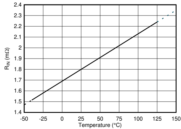
Figure 7-27. Input Conductor Resistance vs. Temperature
