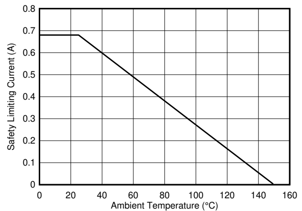
Figure 7-29. Thermal Derating Curve for Safety-Limiting Current, Side 2
