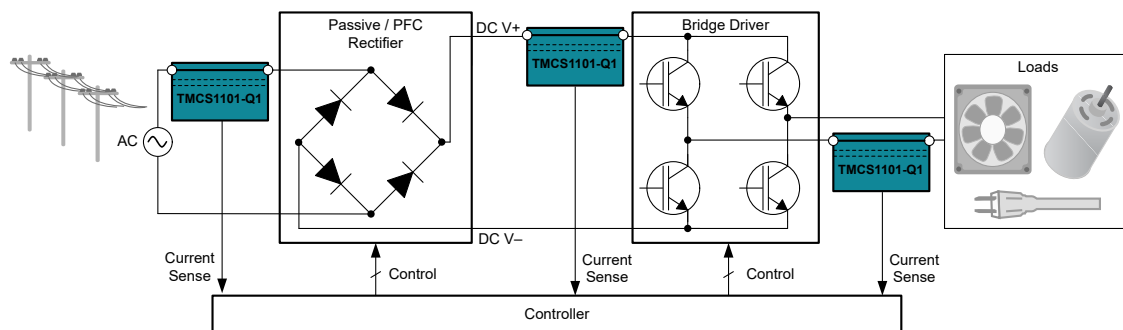
Typical Application
