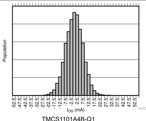
Figure 7-15. Input Offset Current Production Distribution
