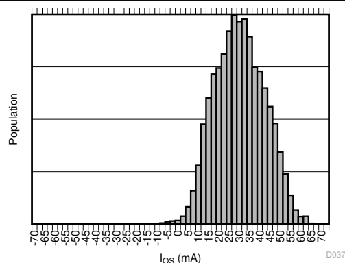
Figure 7-14. Input Offset Current Production Distribution
