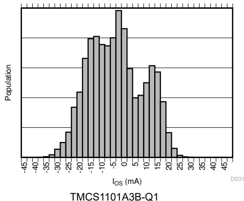
Figure 7-13. Input Offset Current Production Distribution
