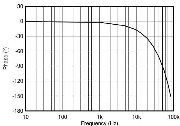
Figure 9-10. Normalized Phase, All Variants
