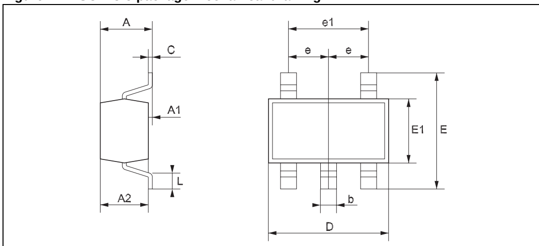
Figure 17. SOT23-5 package mechanical drawing
