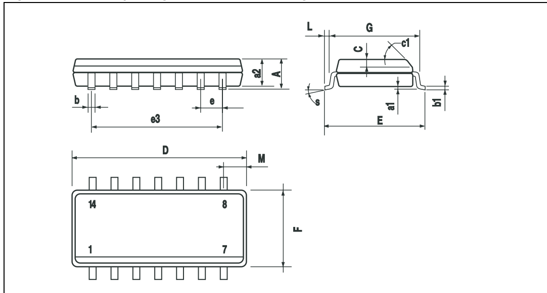
Figure 22. SO-14 package mechanical drawing
