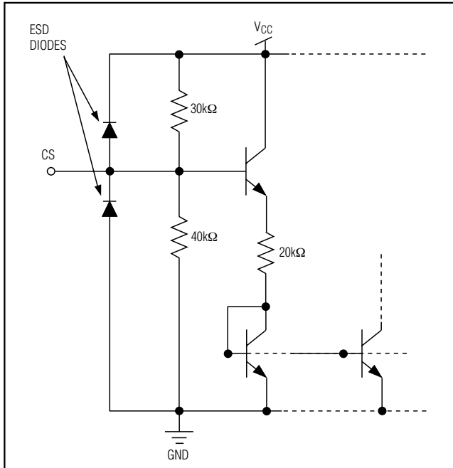
Figure 6. Channel-Select Interface
