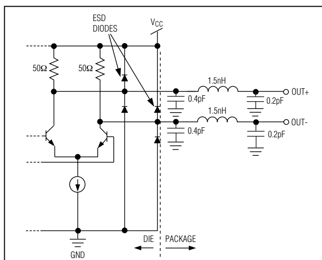
Figure 3. Output Structure
