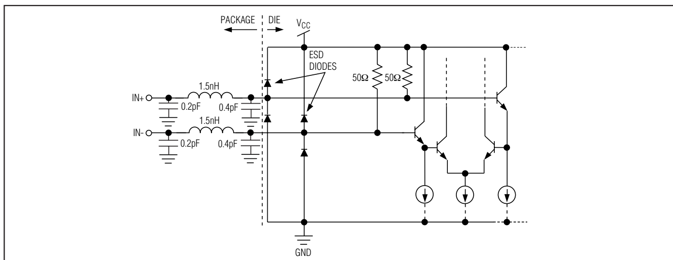
Figure 2. Input Structure
