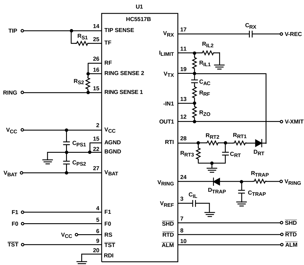
FIGURE 5. TRAPEZOIDAL RINGING APPLICATION CIRCUIT
