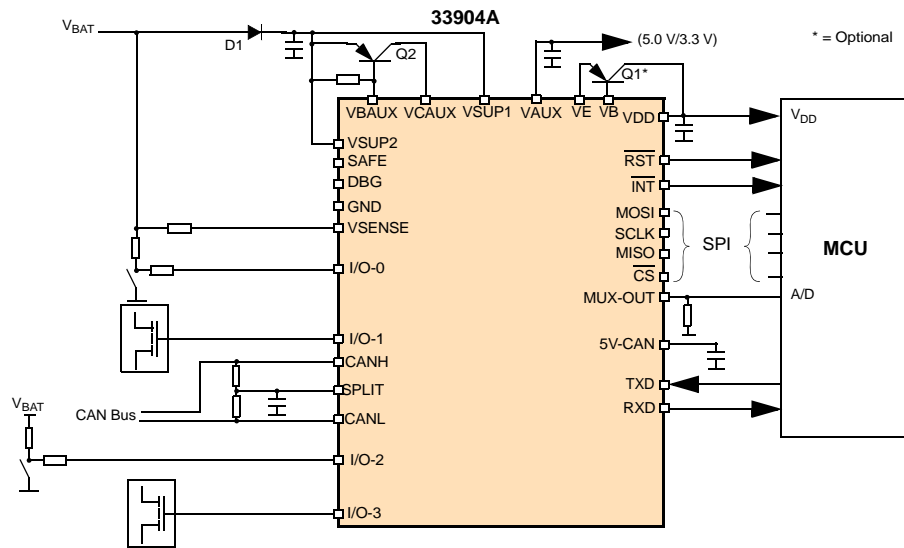
Figure 3. 33904A Simplified Application Diagram
