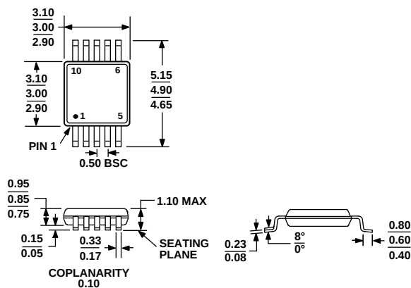
COMPLIANT TO JEDEC STANDARDS MO-187-BA Figure 56. 10-Lead Mini Small Outline Package [MSOP] (RM-10)
