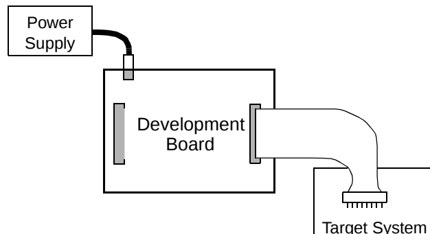
Stand-Alone Environment
