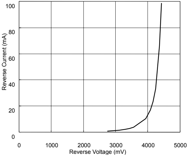
ZD5228A Reverse Current vs Reverse Voltage
