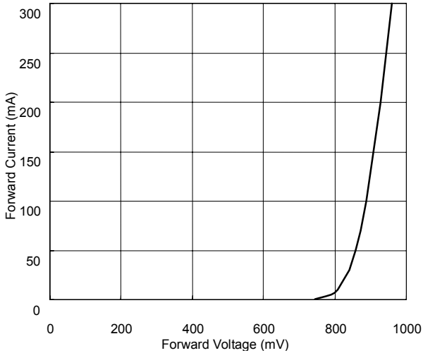
ZD5229A Forward Current vs Forward Voltage
