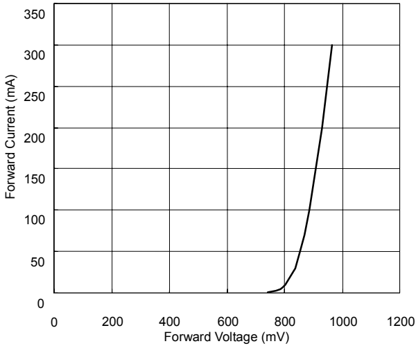
ZD5226A Forward Current vs Forward Voltage
