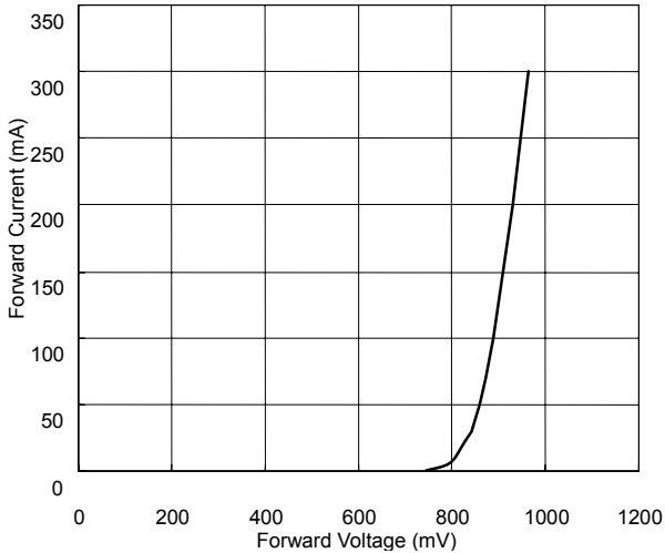
ZD5228A Forward Current vs Forward Voltage
