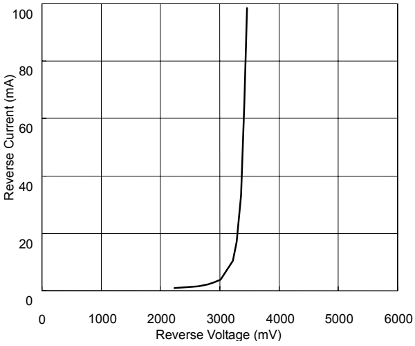
ZD5226A Reverse Current vs Reverse Voltage
