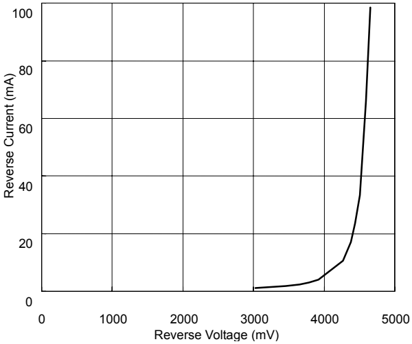
ZD5229A Reverse Current vs Reverse Voltage
