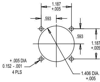
Mounting Layout
