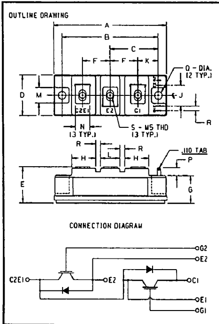
ID226010 Outline Drawing
