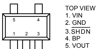
Figure 1. Pin Assignment of APE8805A
