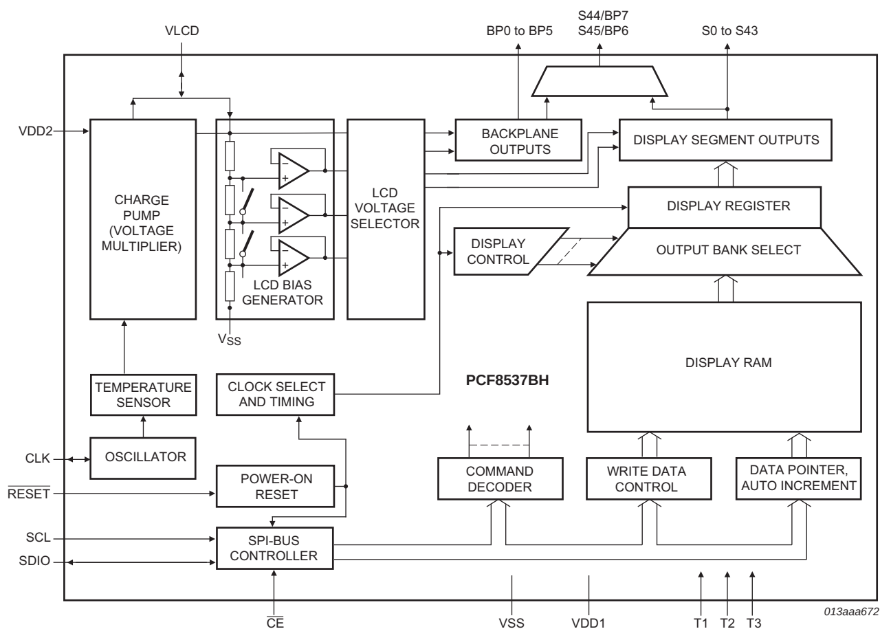
Fig 2. Block diagram of PCF8537BH
