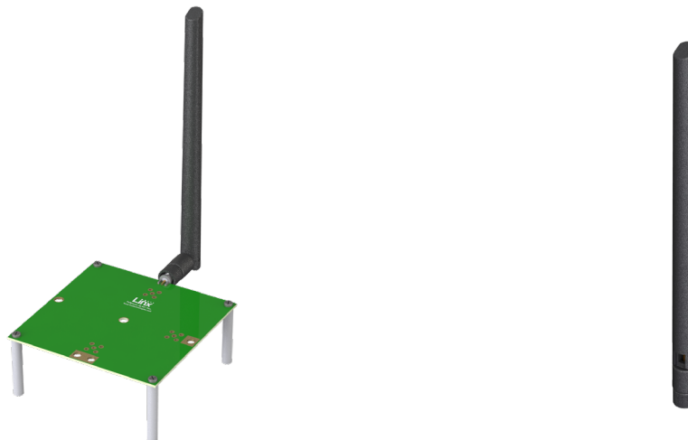
On edge of ground plane, bent 90 degrees
